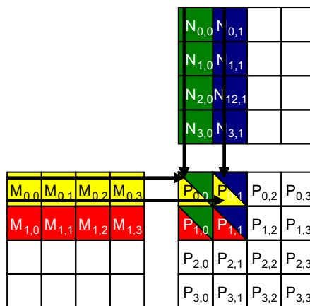
A small example of matrix multiplication. For brevity, We show d\_M[y*Width + x] , d\_N[y*Width + x] , d\_P[y*Width + x] as M_{y,x} , N_{y,x} , P_{y,x} , respectively.
