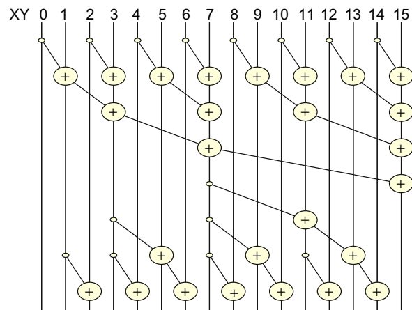
FIGURE 9.5 Basic idea of a work-efficient parallel scan algorithm.
