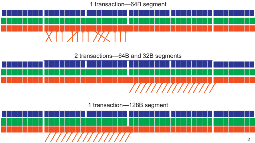
FIGURE B.2 Memory coalescing in compute 1.2 and higher.
