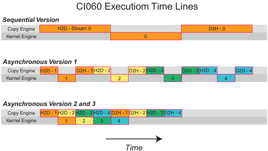
FIGURE 17.1 Data transfer and kernel execution timing for the sequential and asynchronous versions when there is only one copy engine.
